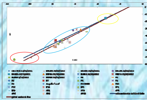
Events analysed referred to the monitoring stations.
