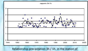
Relationship precipitation 3h / 1h, in the station of Codigoro.
