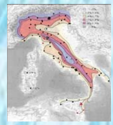
Variation of the isotopic composition of rainwater. (Longinelli and Selmo, 2003)
